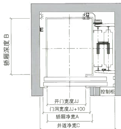
Hoistway plan (Counterweight side placement)
