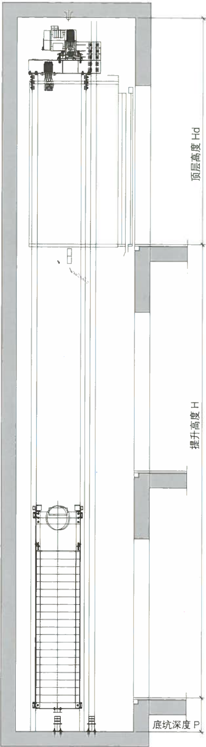
Hoistway elevation (Counterweight side placement)
