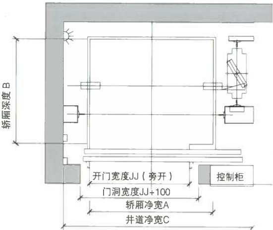
Hoistway plan (Counterweight side placement)
