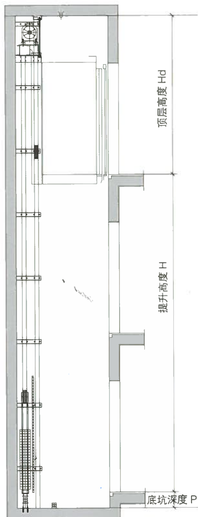
Hoistway elevation (Counterweight rear placement)
