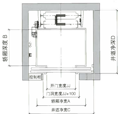
Hoistway plan (Counterweight rear placement)
